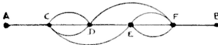
FIG. 23.—Simplified Diagram of Fig. 22.
