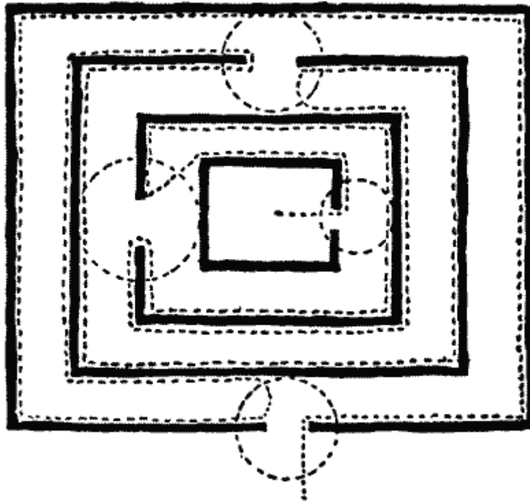
FIG. 20.—M. Tremaux's Method of Solution.
